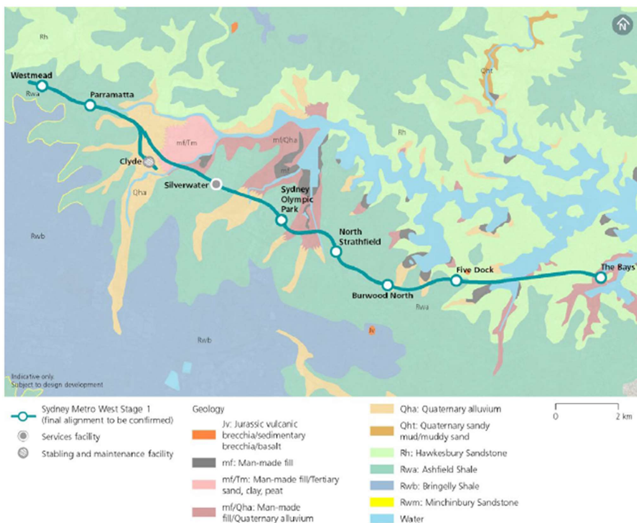
FIGURE 1: GEOLOGICAL FORMATIONS FOR THE CTP
