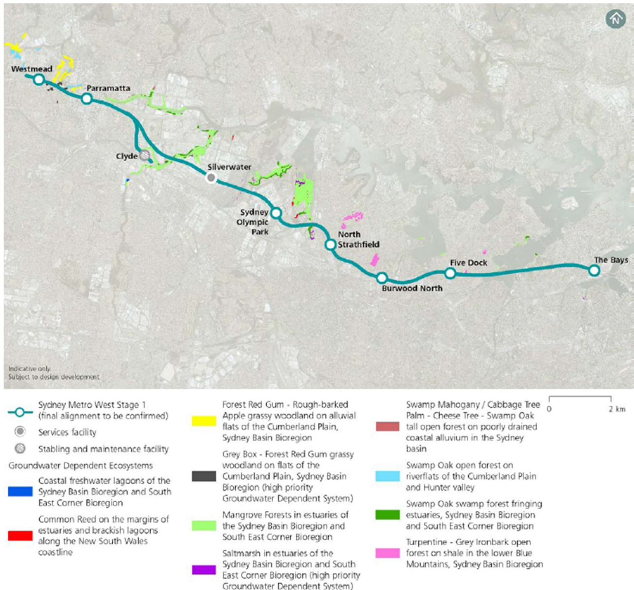
FIGURE 2: GROUNDWATER DEPENDENT ECOSYSTEMS
